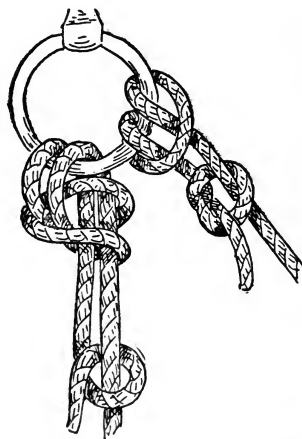
FIG. 56.—Larks' heads and running noose.
